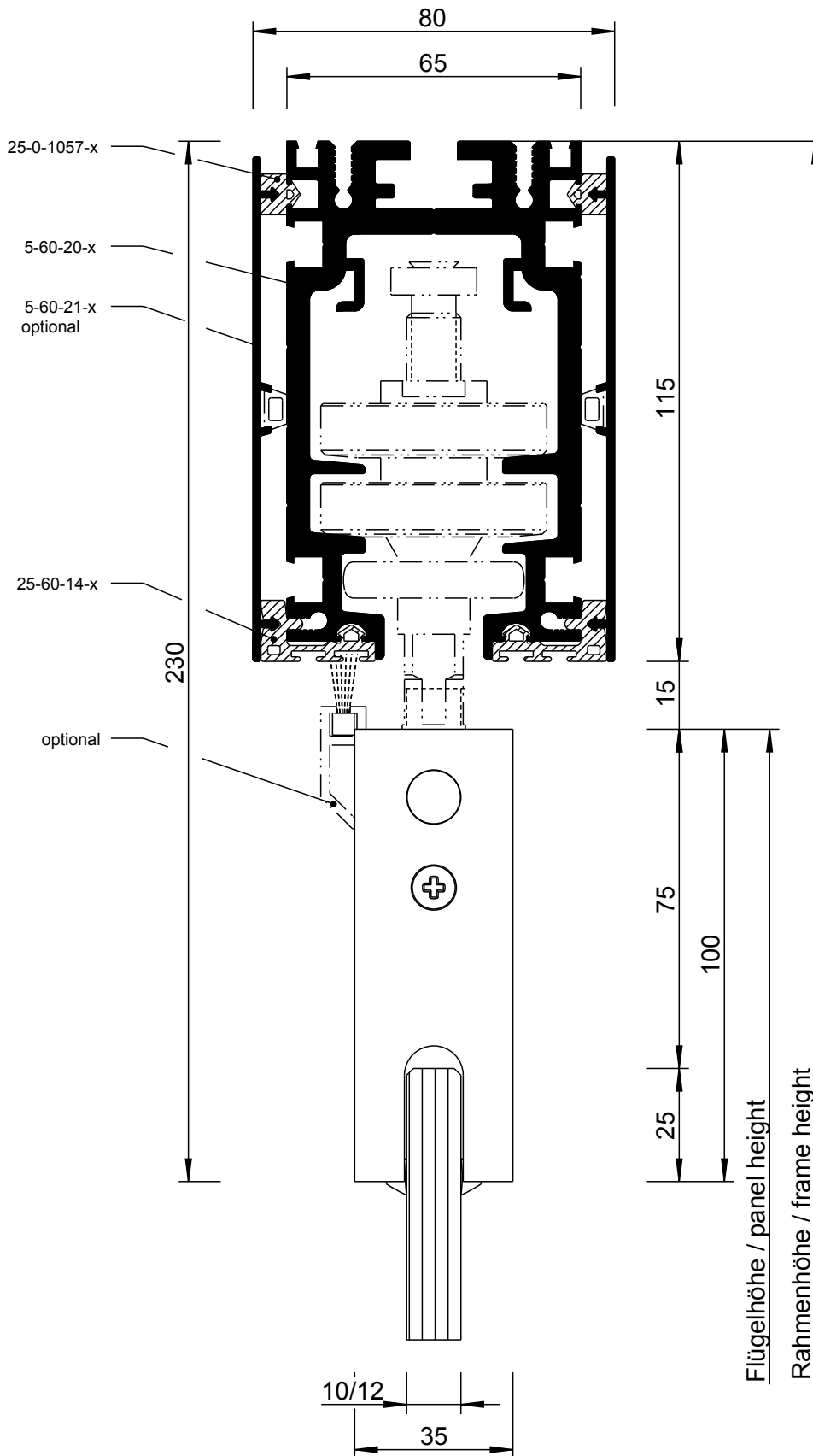
Detail GGHSW-1-2
